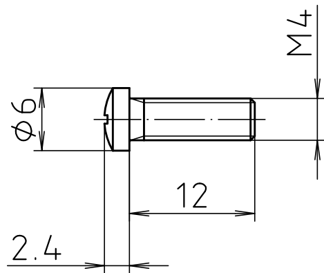
SHR Z M4x12 SO (BFS 0400)
